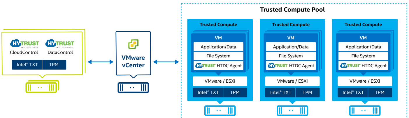
Figure 3. Interconnection of HTCC and HTDC to trusted compute pools.
