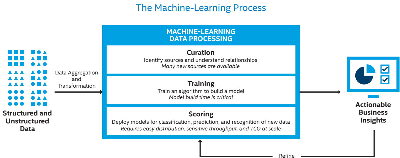
Figure 3. The basics of machine learning include data ingestion, data analysis and model training, and results generation. Self-learning capabilities continuously improve the model's accuracy.
