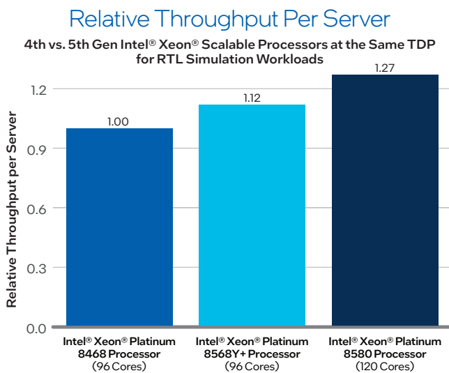
Figure 7. EDA throughput of high-core-count 4th and 5th Gen Intel® Xeon® Platinum processors at the same TDP.
