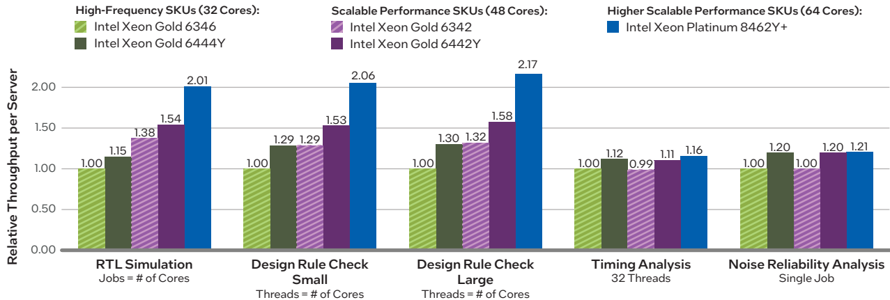
Figure 2. 4th Generation Intel® Xeon® Scalable processor vs. 3rd Generation Intel Xeon Scalable processor: More cores provide more system throughput for EDA workloads. Note: Same application binary used across all of the platforms. 1
