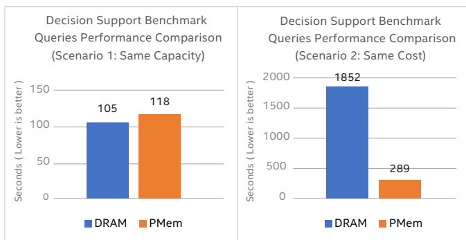
Figure 3. DRAM and Intel® Optane™ PMem Comparison Tests 1
